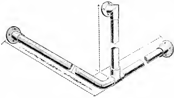
Fig. 3578. SECTION CURTAIN-ROD.
